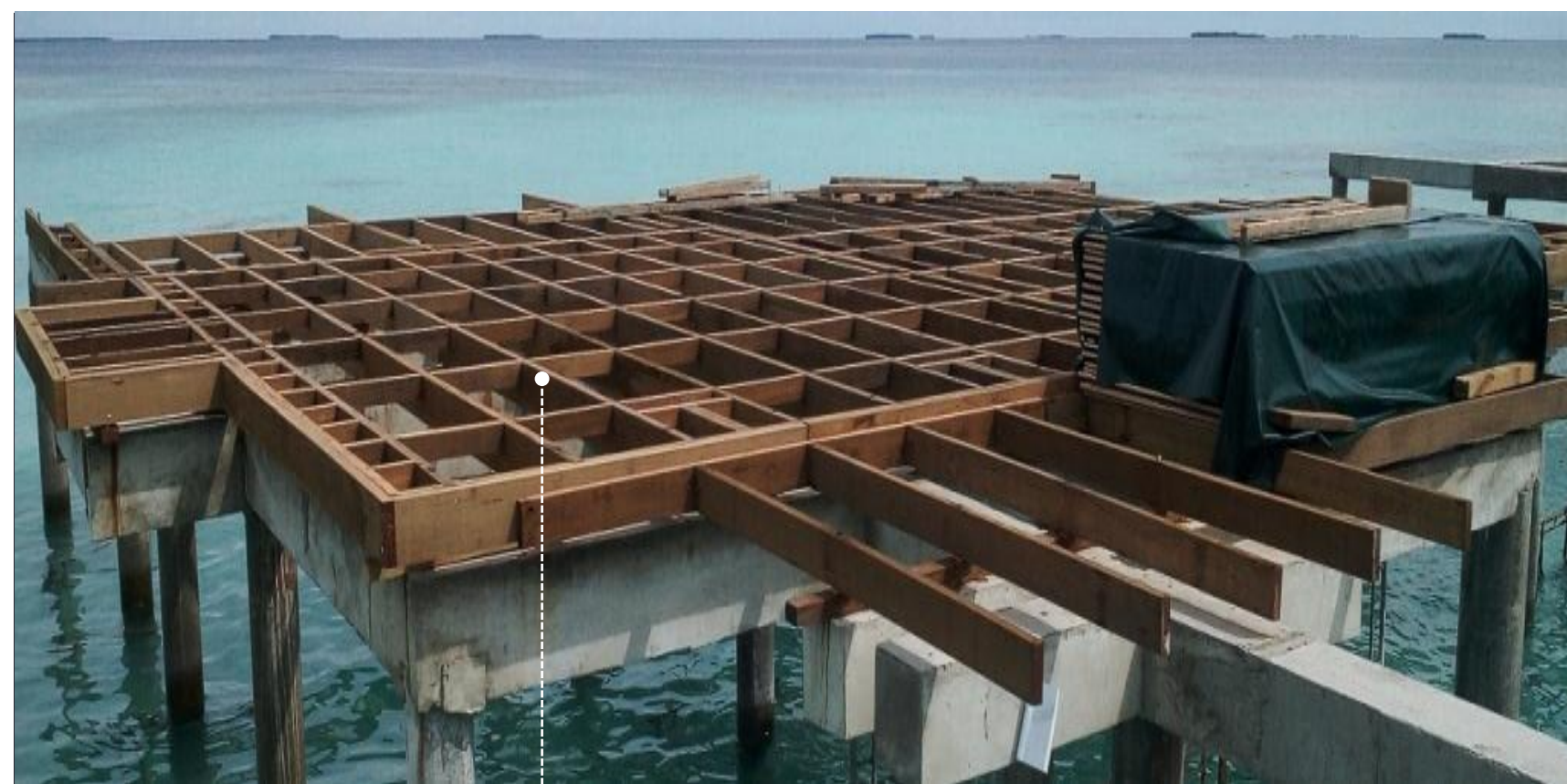
Timber Joists and Noggings
