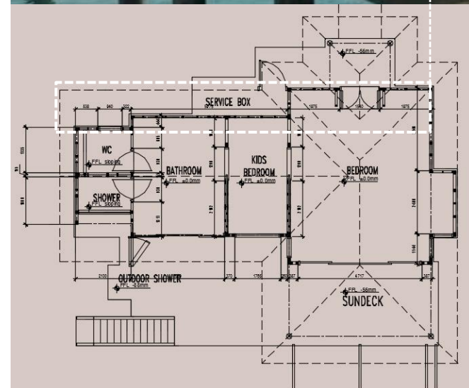
MODULAR WALL FRAME LAYOUT PLAN
