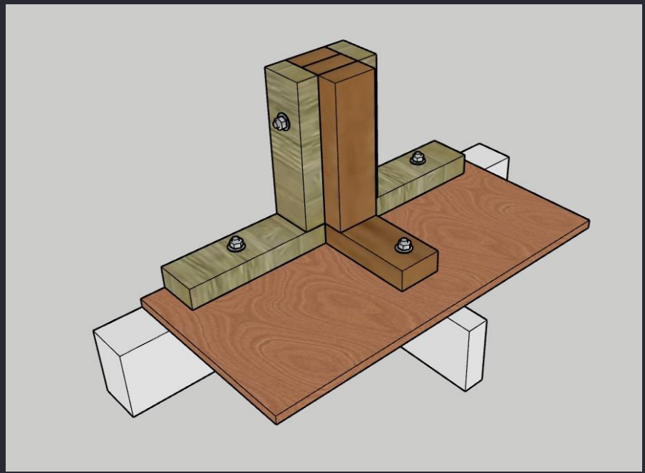
TYPICAL WALL FRAME CONNECTION DETAIL
