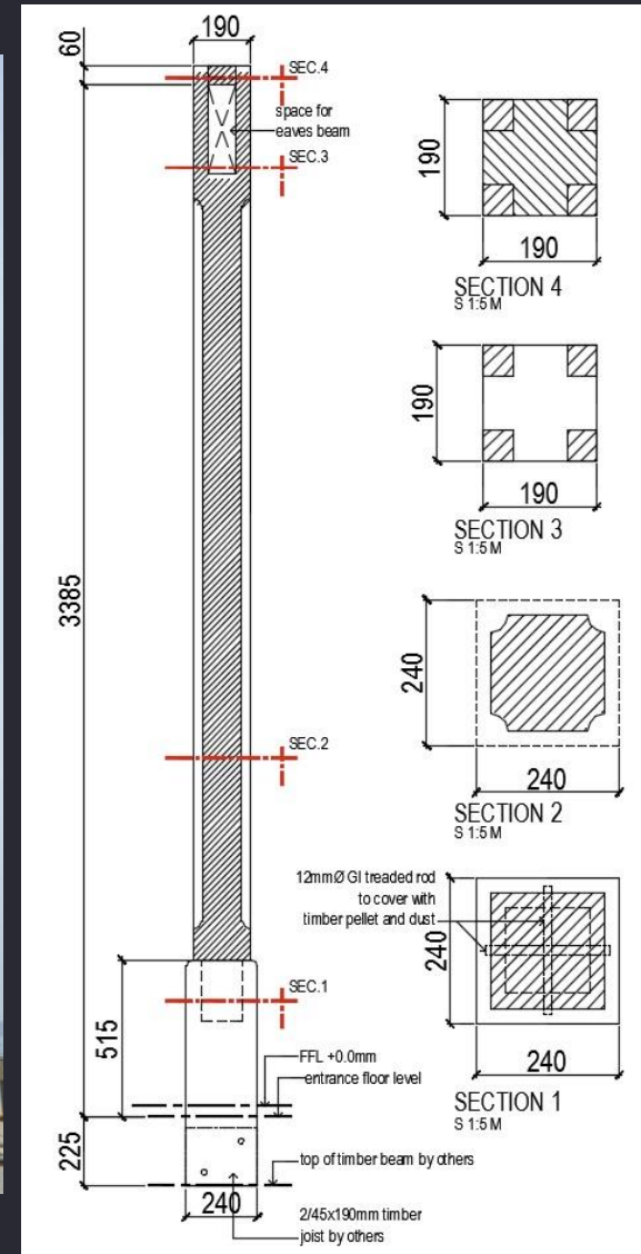
TYPICAL PROFILED TIMBER COLUMN
